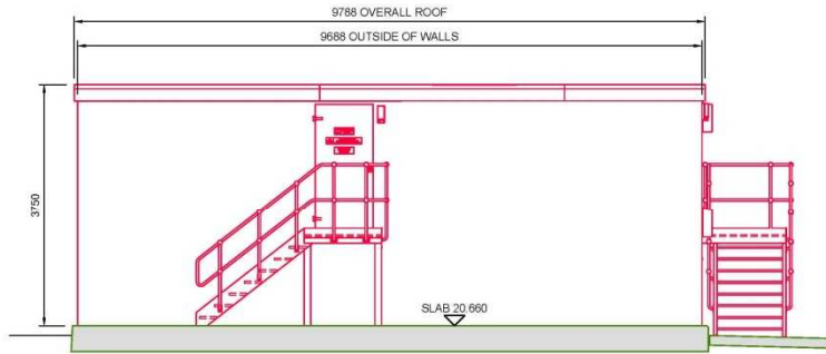
ELEVATION VIEW ON A
