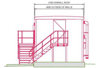
ELEVATION VIEW ON D
