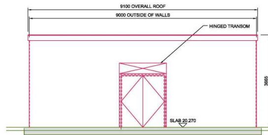
ELEVATION VIEW ON A
