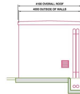
ELEVATION VIEW ON D
