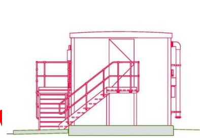
ELEVATION VIEW ON B
