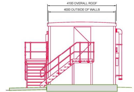
ELEVATION VIEW ON D
