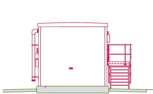
ELEVATION VIEW ON B
