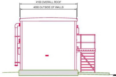
ELEVATION VIEW ON D
