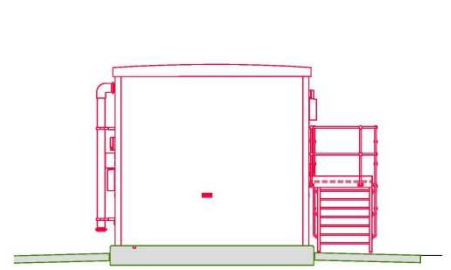
ELEVATION VIEW ON B
