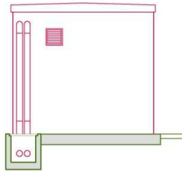
ELEVATION VIEW ON B
